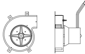
Draft Inducer
